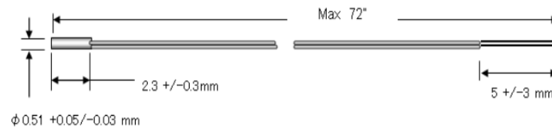
F Micro Thermistor Dimensions (example)
