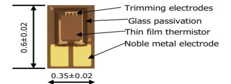
F \mu thermistor chip
